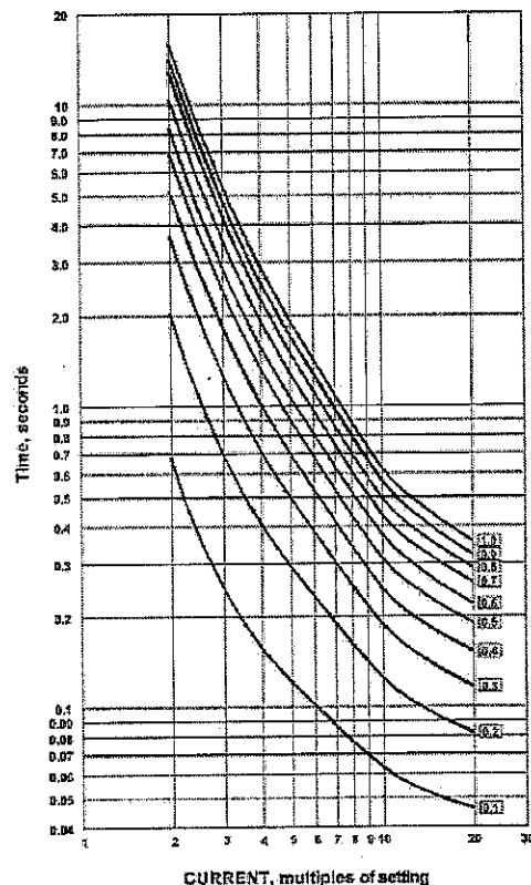
Fig.1 Time / Current Characteristic
